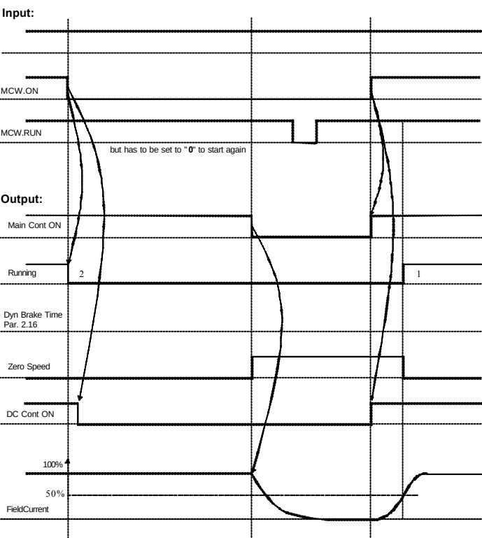
Fig. 3 Stopping via fault signal in case of Dynamik Braking
